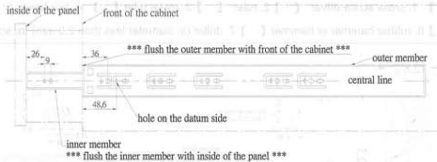
FIG.1 OUTER MEMBER
