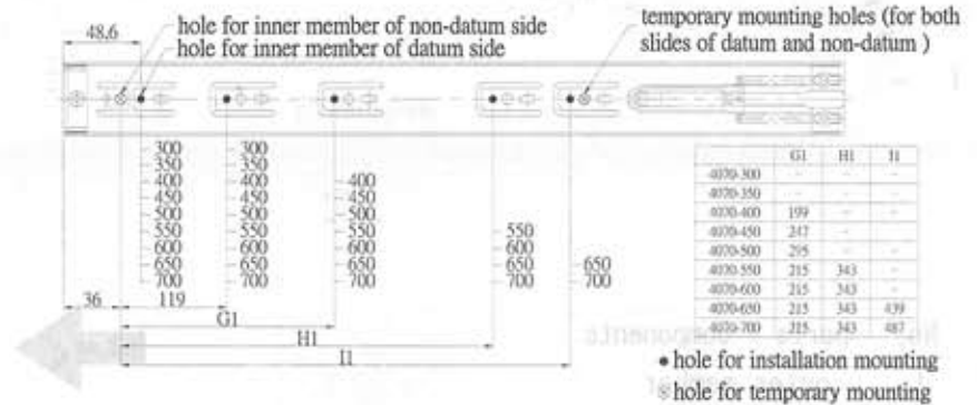
FIG.1 OUTER MEMBER
